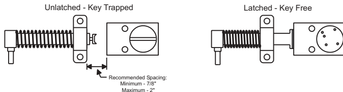
Optional DM Latch Bolt with Spring and Mounting Bracket
