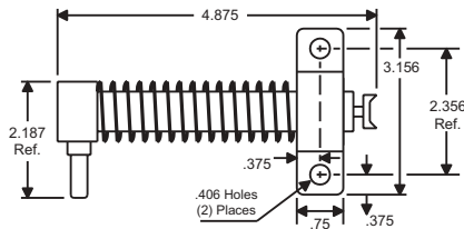
Optional DM Latch Bolt with Spring and Mounting Bracket
