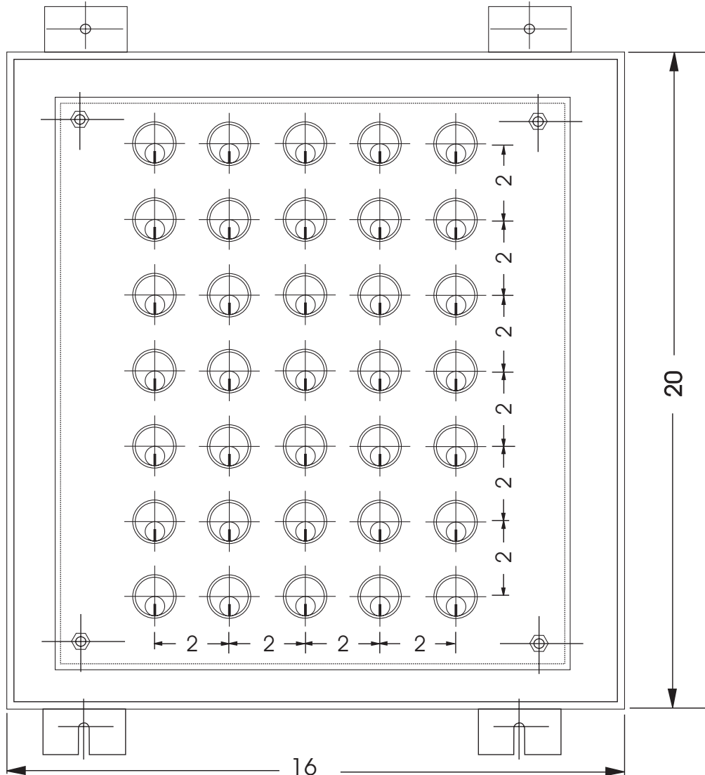
Transfer Panel Catalog #227-856-005 shown in drawing.
